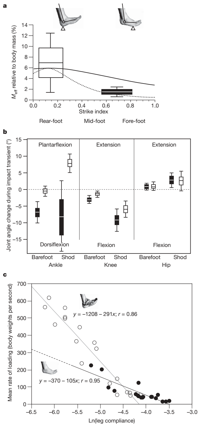
Figure 3 | Differences during impact between shod RFS runners (group 1) and barefoot FFS runners (group 3) at approximately 4 m s -1 . a , Predicted (lines) and measured (boxes) effective mass, M_{\text{eff}} , relative to body mass, versus foot length at impact (strike index) for FFS and RFS runners in the barefoot condition (Methods). The solid and dotted lines show predicted M_{\text{eff}} values for infinitely stiff and infinitely compliant ankles, respectively, at different centres of pressure. b , During the impact period, FFS runners (filled boxes) dorsiflex the ankle rather than plantarflexing it, and have more ankle and knee flexion than do RFS runners (open boxes). Boxes, mean \pm s.d.; whiskers, mean \pm 2 s.d. c , Overall dimensionless leg compliance (natural logarithm) during the impact-transient period (ratio of vertical hip drop relative to leg length at 90% of impact transient peak, normalized by body weight) relative to the rate of impact loading (body weights per second) for RFS runners (open circles) and FFS runners (filled circles) (shod and unshod conditions). Compliance is greater and is correlated with lower rates of loading in FFS impacts than in RFS impacts (plotted lines determined by least-squares regression; r , Pearson's correlation coefficient).
