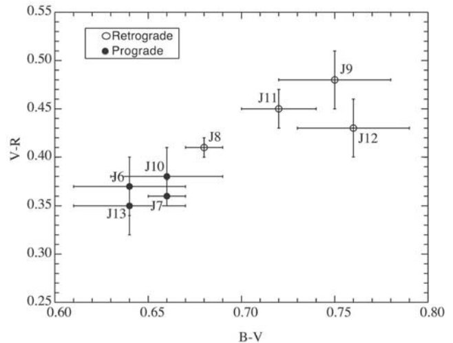
Figure 12.7. Optical colors of the eight brightest irregular satellites, from Rettig et al. (2001).
