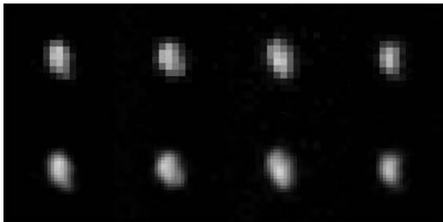
Figure 12.3. The disk of Himalia illuminated from the left at a phase angle of 70^\circ . and observed by the Cassini ISS over \sim 4.5 hours. One unprocessed image from each of four observation sequences is shown in the top row. The observation times were (from left to right): 18 December 2000, 20:30 UTC, 22:00 UTC, 23:30 UTC, and 19 December 2000, 01:04. The bottom row shows the same data, but smoothed by bicubic interpolation. From Porco et al. (2003).
